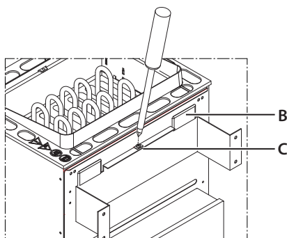
B. Mounting slots
